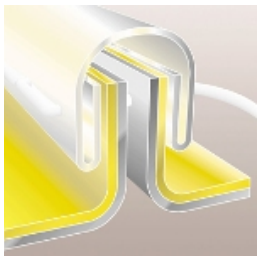
Bound Seam
